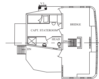
CO2 DECK - BRIDGE
