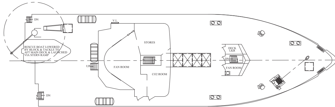
01 DECK
